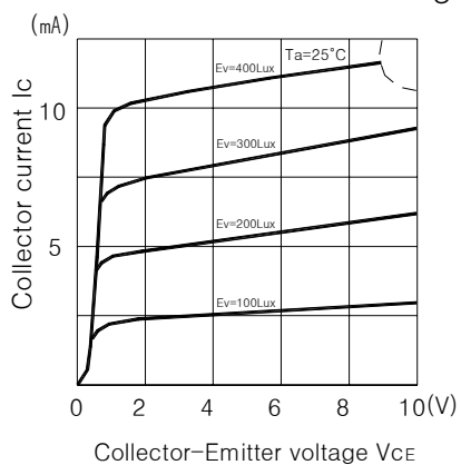
■ Collector current Vs Collector-Emmitter voltage
