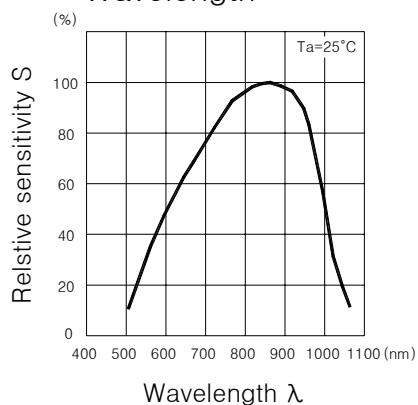
■ Relative sensitivity Vs Wavelength
